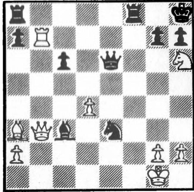
121 After 20...Rxf8
